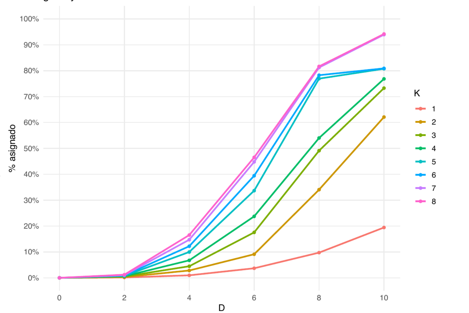
greedy – ext – 10–32
