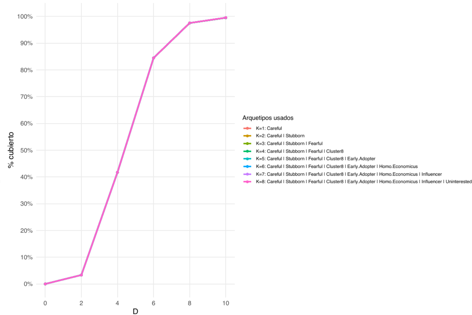
greedy – pos – 10–32
