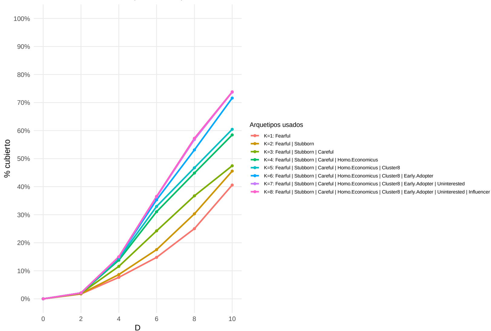
kmeans – ext – 10–32 (orden D=4)
