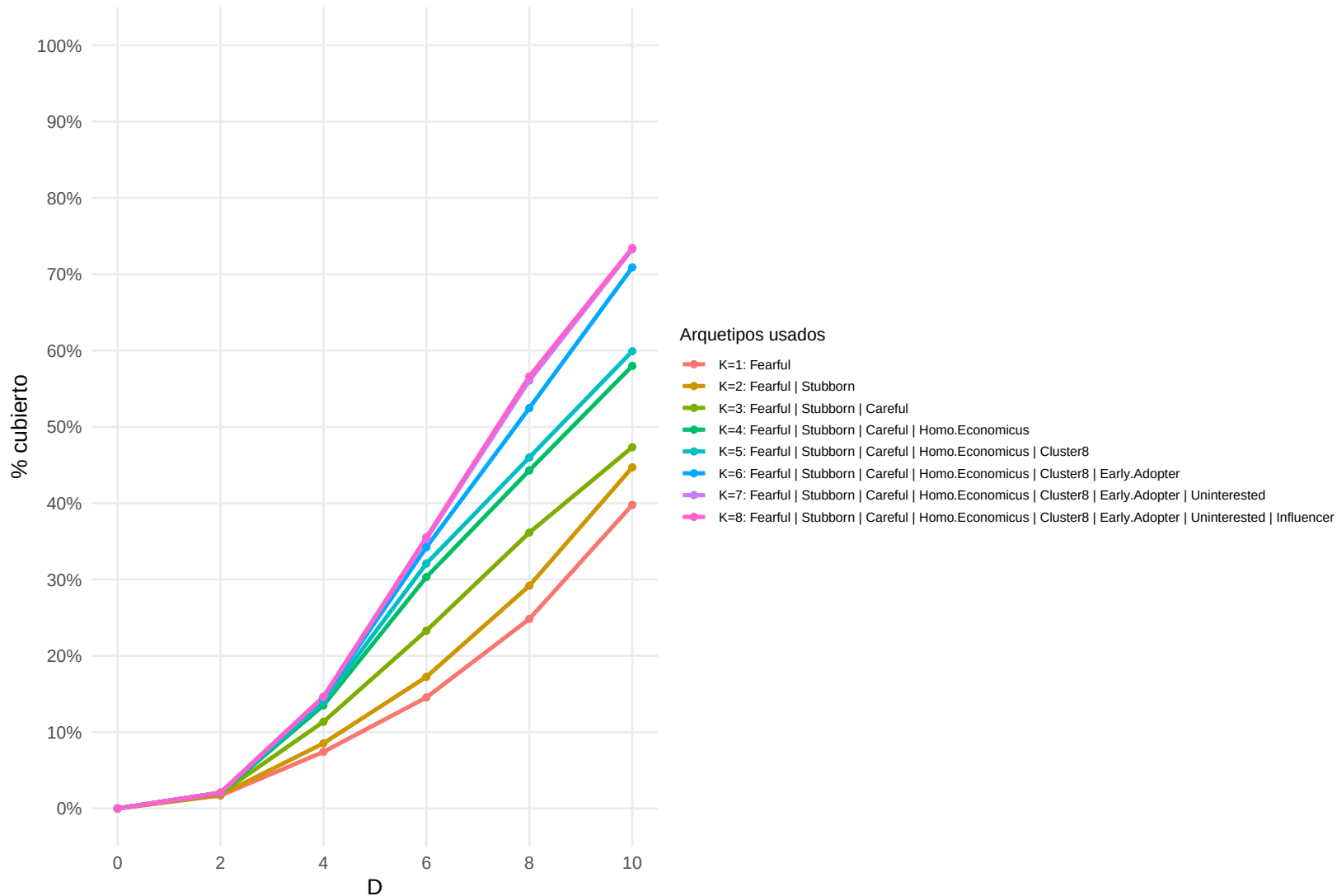
kmeans – ext – 100–32 (orden D=4)
