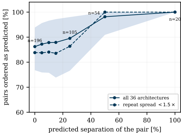
(b) n: architecture pairs; band: 95% architecture-level bootstrap
