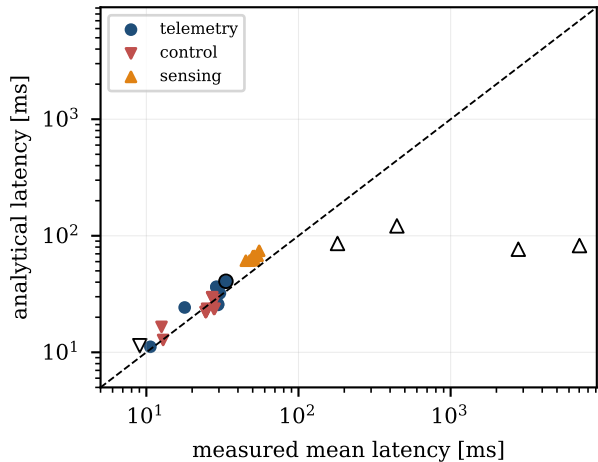
(a) open markers: repeat spread \geq 1.5 \times
