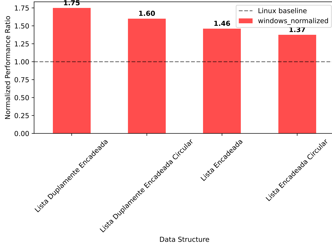
Windows Performance Relative to Linux (Linux baseline = 1.0)
