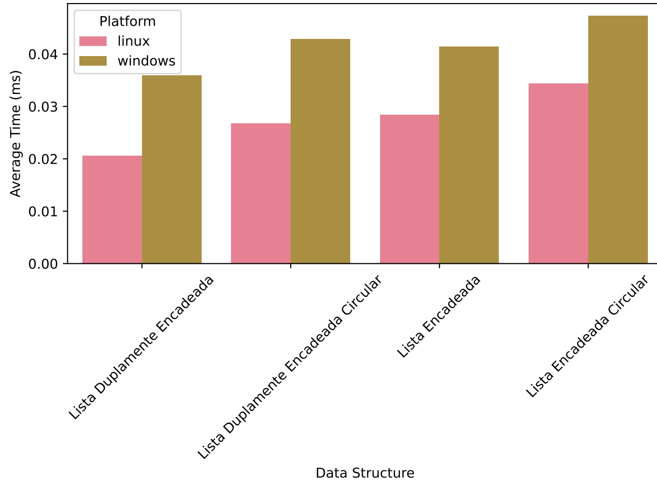
Average Execution Time by Data Structure
