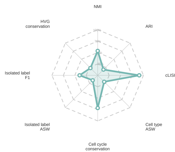
ComBat
