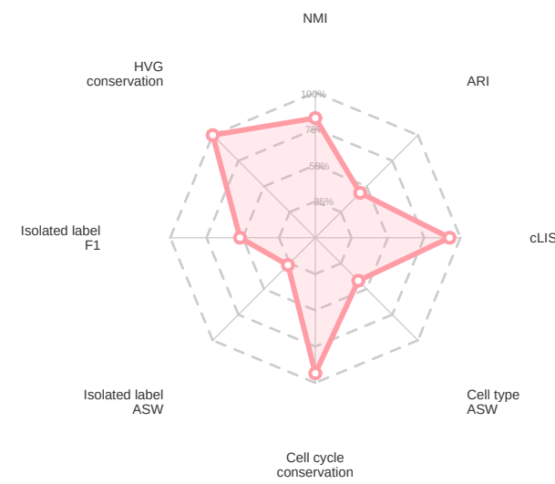
fastMNN
