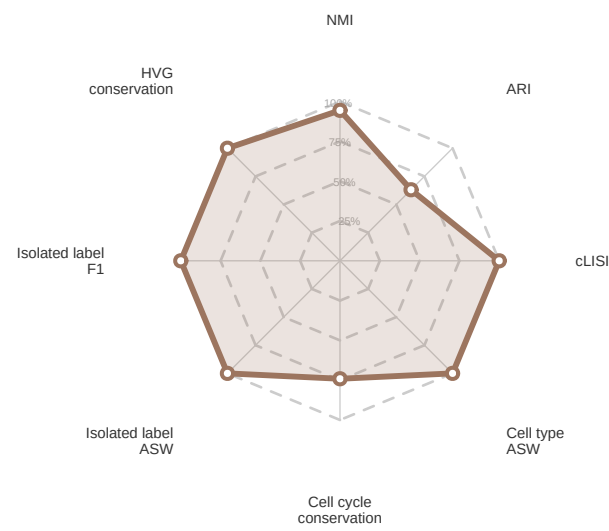
scGen
