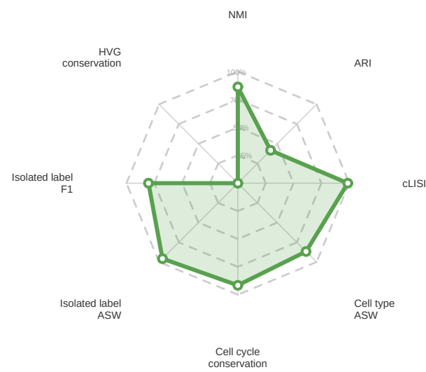
Scanorama
