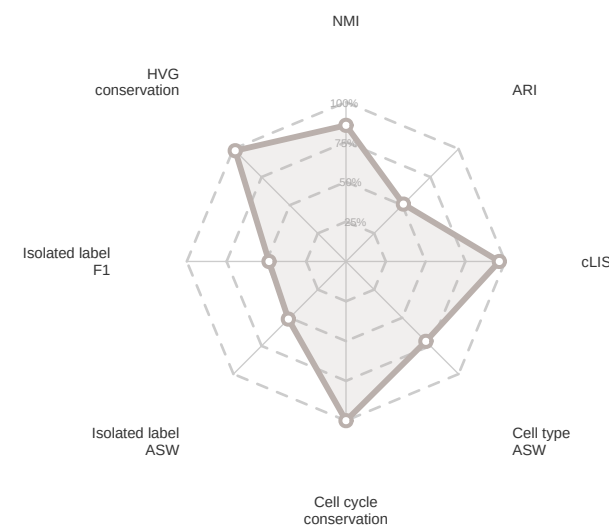
Harmony
