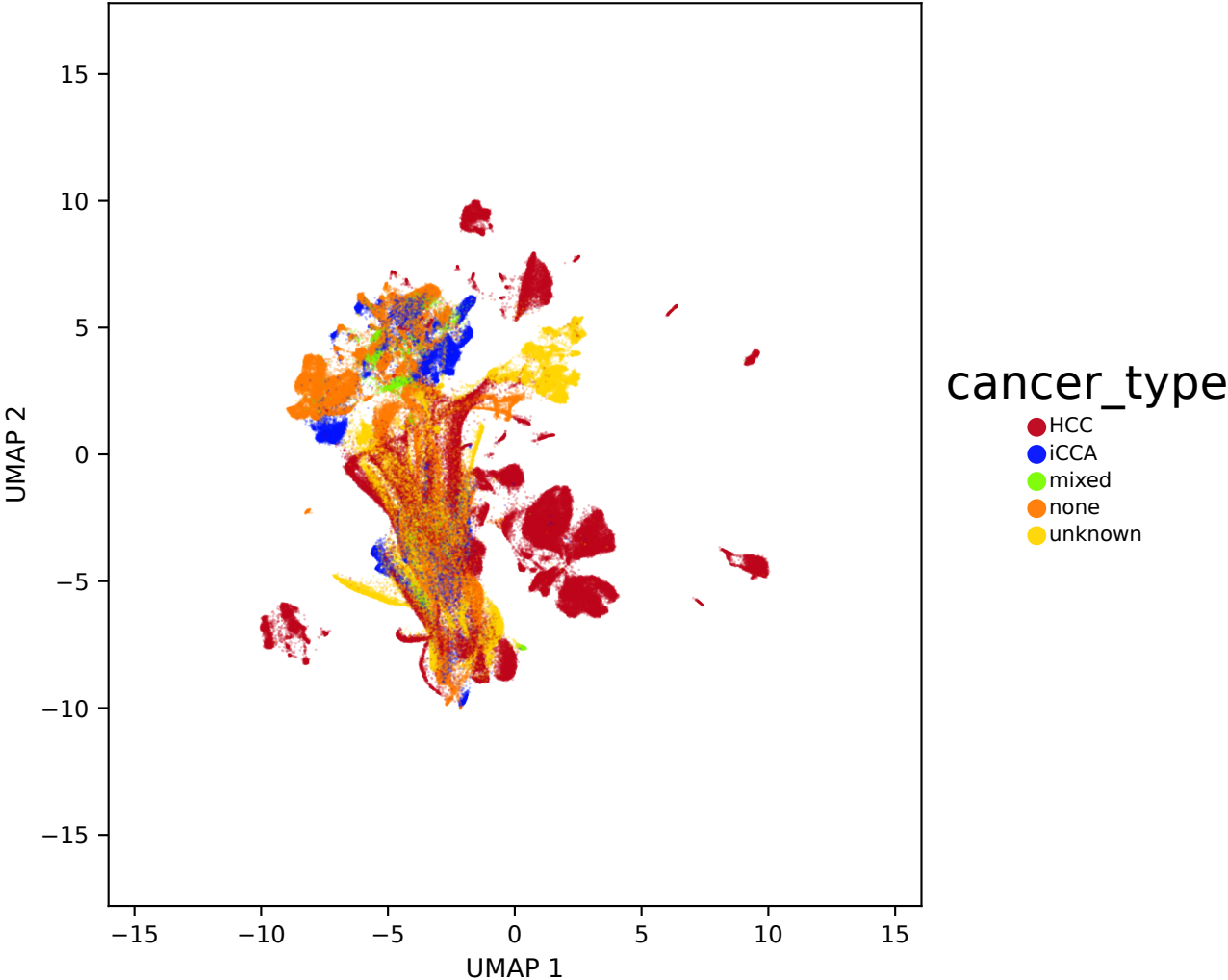
ComBat — combat_full_hvg_seed0 (n=199,996) — cancer type
