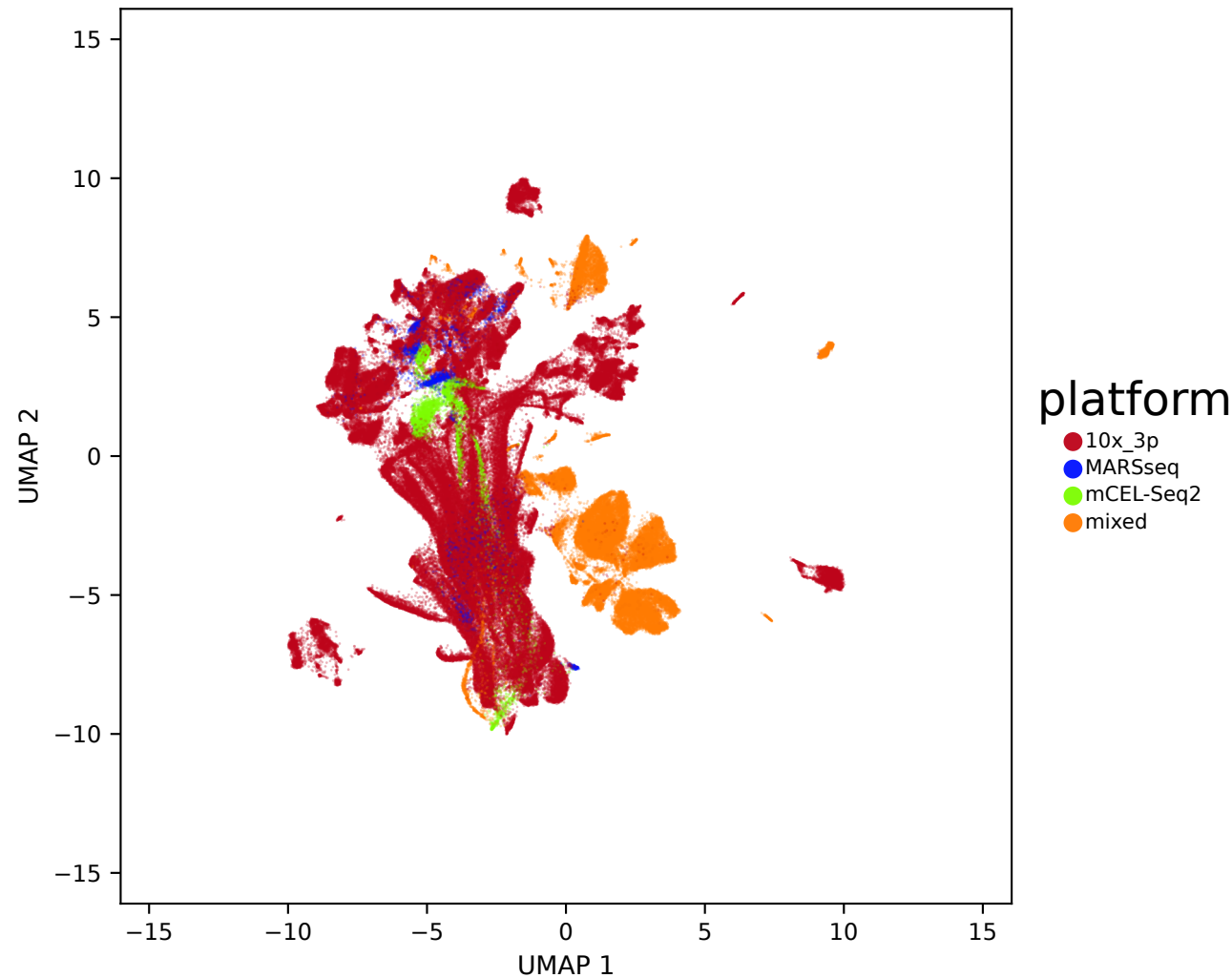
ComBat — combat_full_hvg_seed0 (n=199,996) — platform
