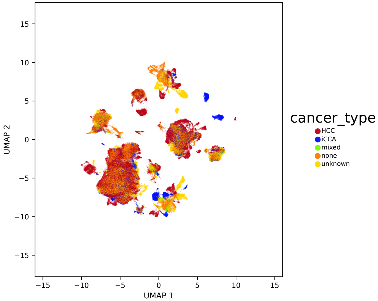
Harmony — harmony_full_hvg_seed0 (n=199,996) — cancer type
