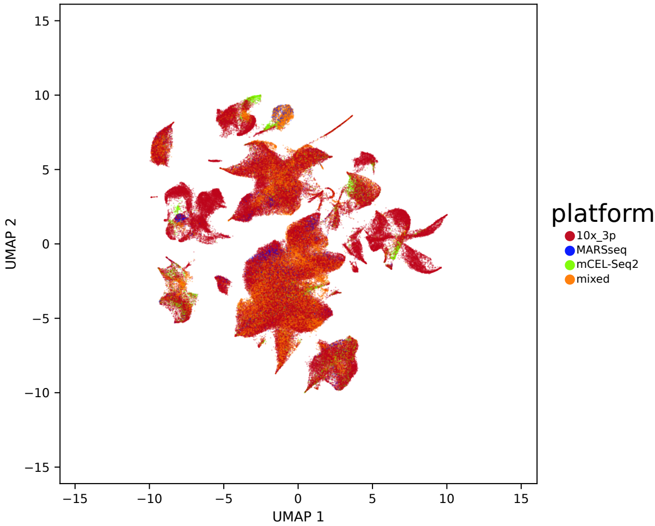
LIGER (external HVGs, full raw panel) — liger_full_hvg_seed0 — platform
