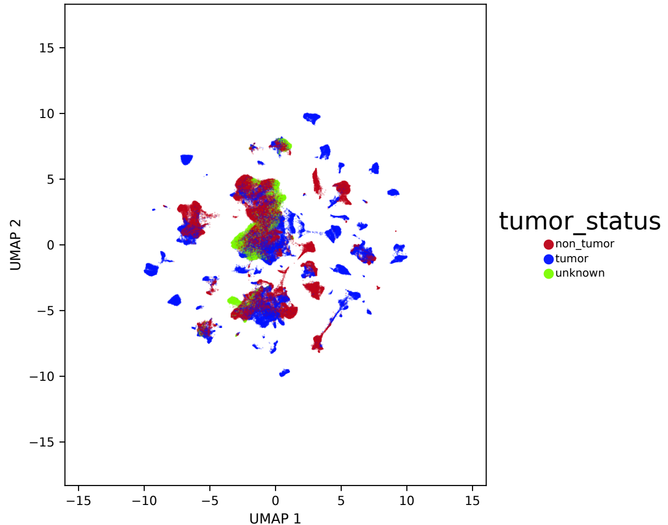
Scanorama — scanorama_full_hvg_seed0 (n=199,996) — tumor status
