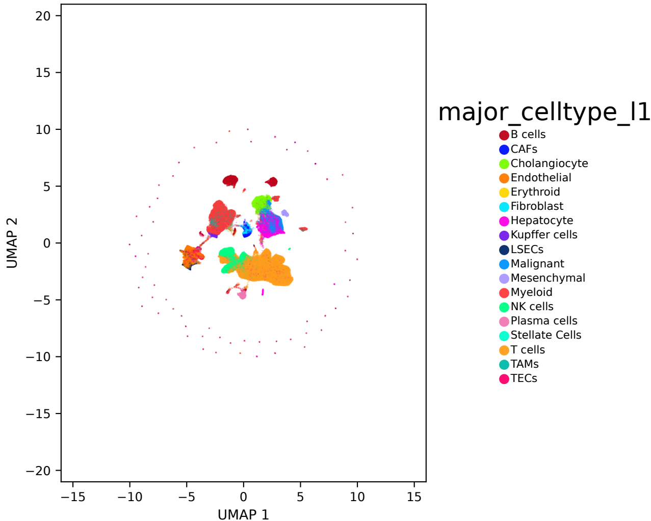
scANVI — scanvi_full_hvg_seed0 (n=199,996) — major celltype l1
