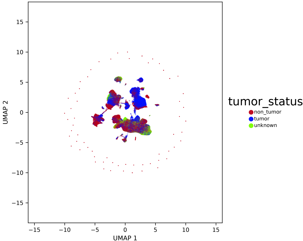
scANVI — scanvi_full_hvg_seed0 (n=199,996) — tumor status
