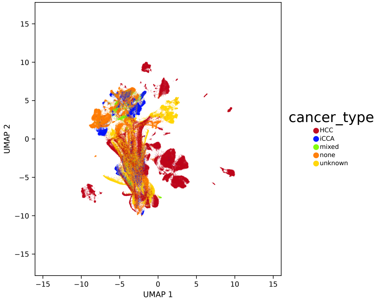
ComBat — combat_parallel6_hvg_seed0 (n=199996) — cancer type
