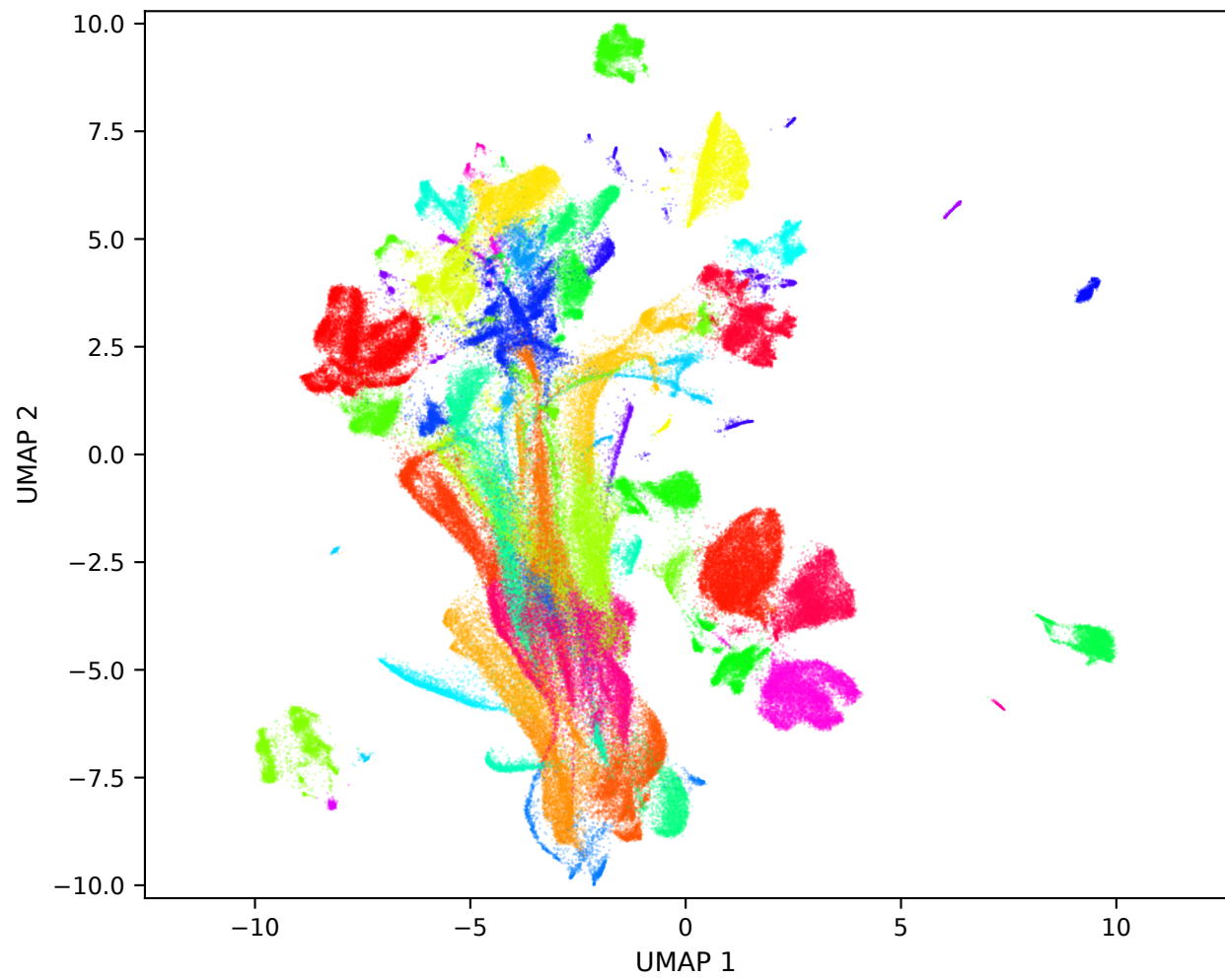
ComBat — combat_parallel6_hvg_seed0 (n=199996) — leiden combat_parallel6_hvg_seed0
