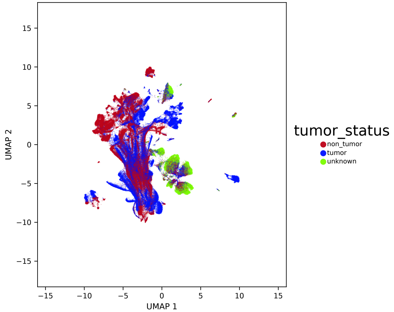
ComBat — combat_parallel6_hvg_seed0 (n=199996) — tumor status
