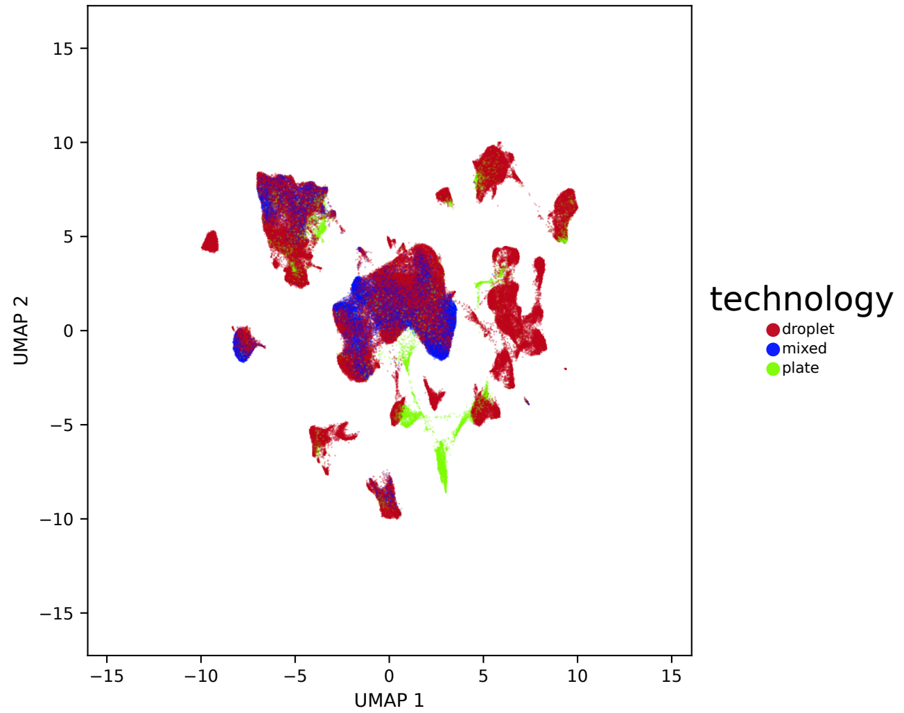
fastMNN — fastmnn_fastmnn_seurat_hvg_seed0 (n=199996) — technology
