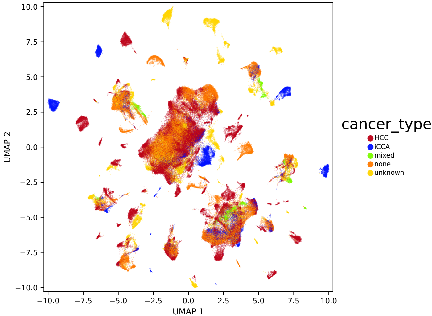
Scanorama — scanorama_full_hvg_seed0 (n=199996) — cancer type
