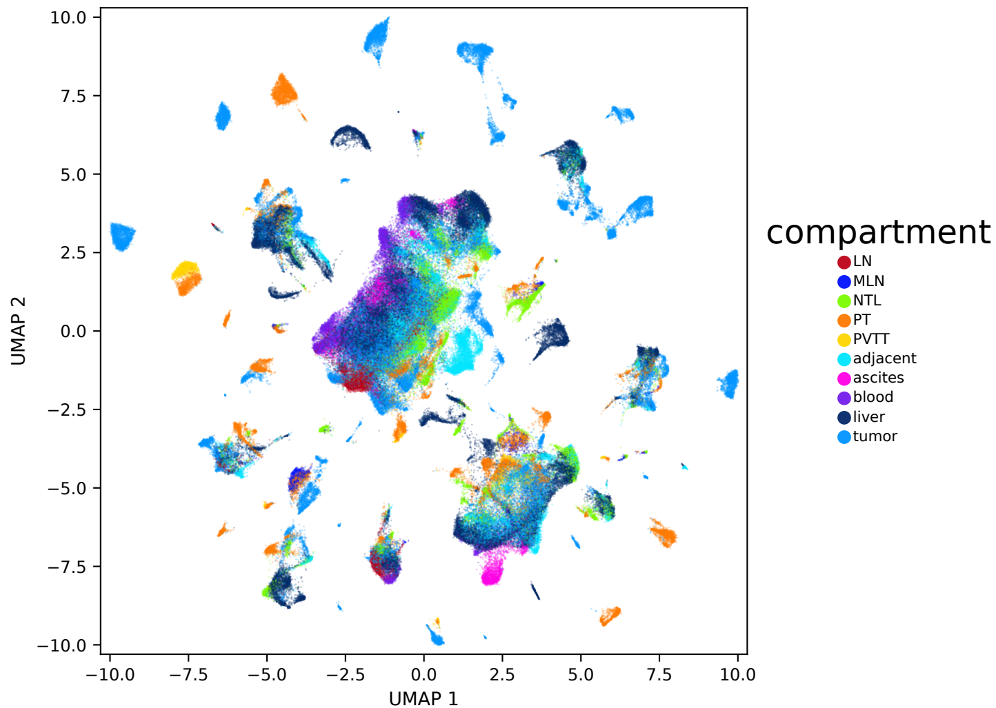
Scanorama — scanorama_full_hvg_seed0 (n=199996) — compartment
