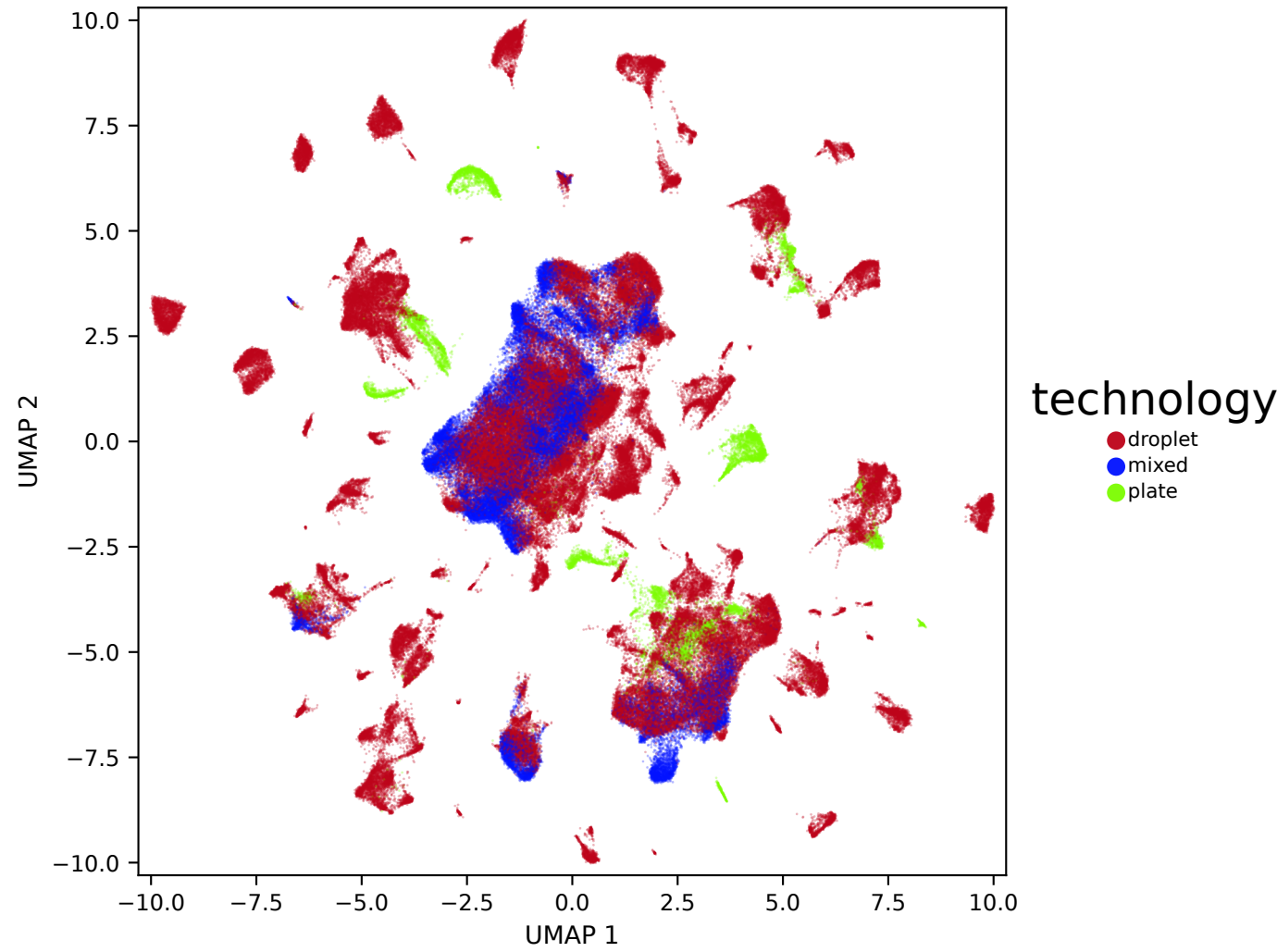
Scanorama — scanorama_full_hvg_seed0 (n=199996) — technology
