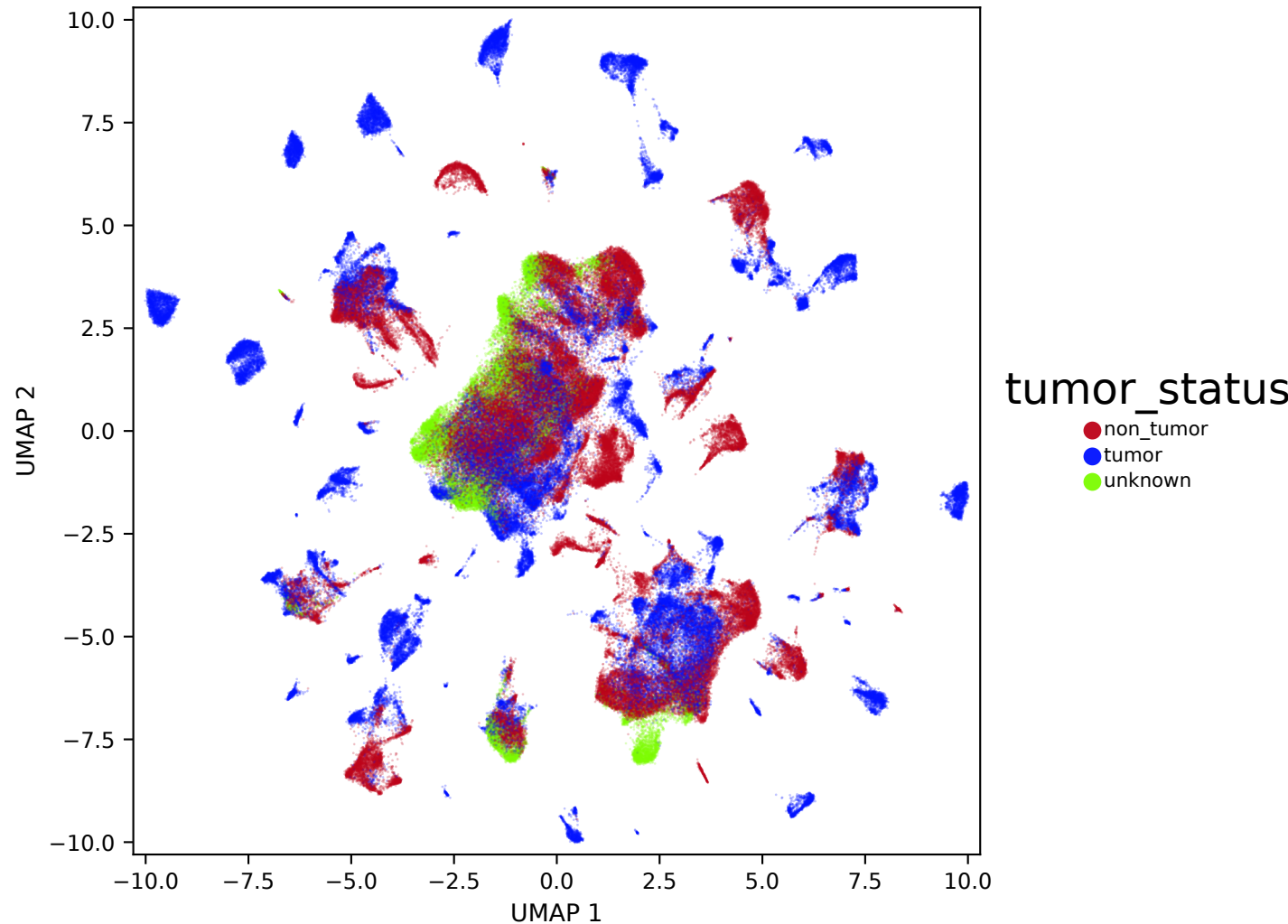
Scanorama — scanorama_full_hvg_seed0 (n=199996) — tumor status
