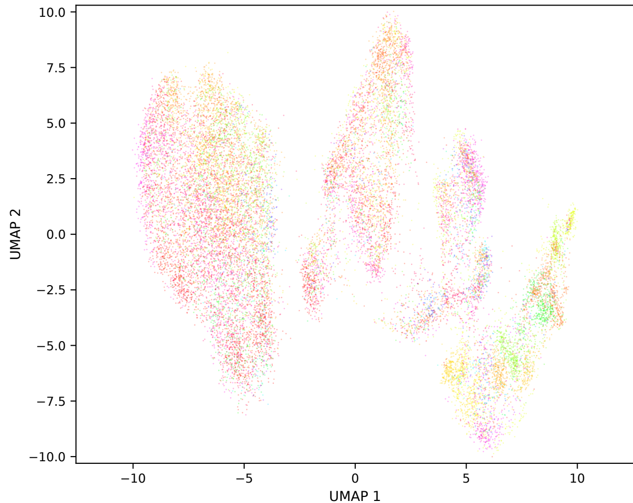
BBKNN — esraa_bbknn_smoke (n=19,997) — donor id
