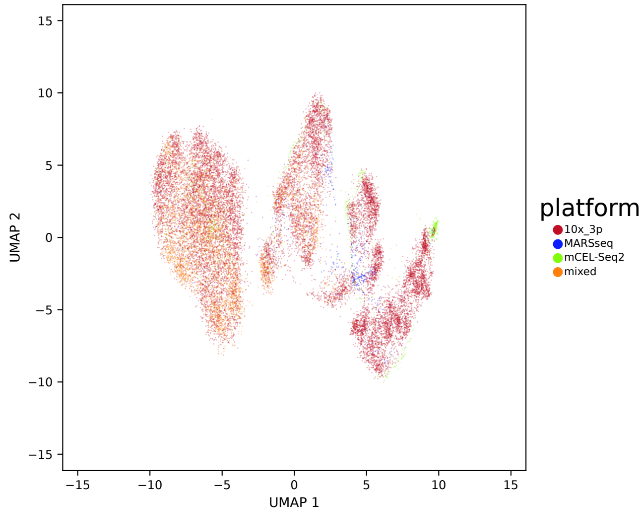
BBKNN — esraa_bbknn_smoke (n=19,997) — platform
