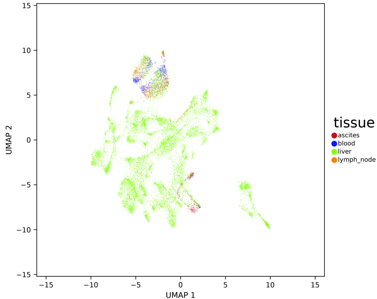
ComBat — combat (n=19,997) — tissue
