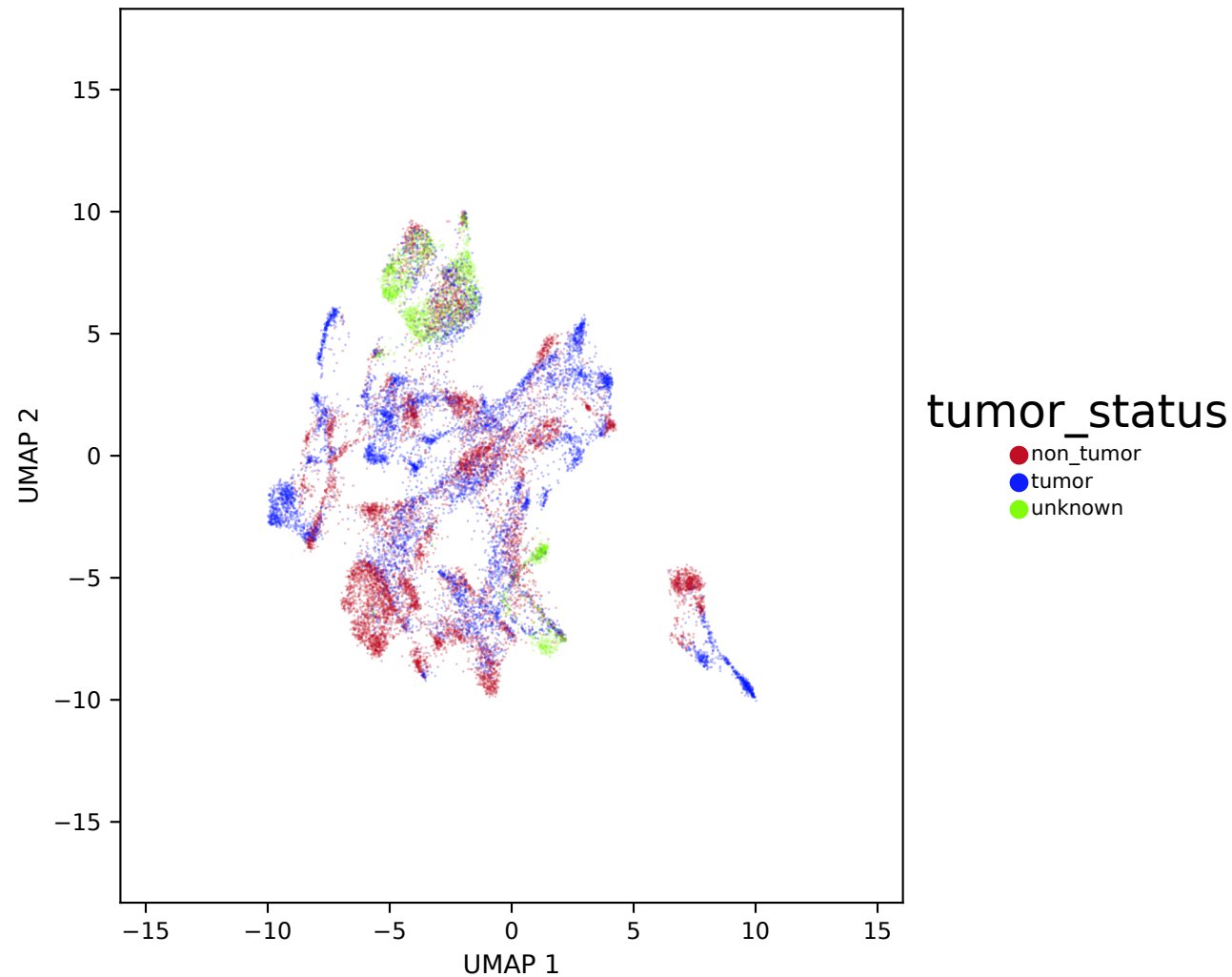
ComBat — combat (n=19,997) — tumor status
