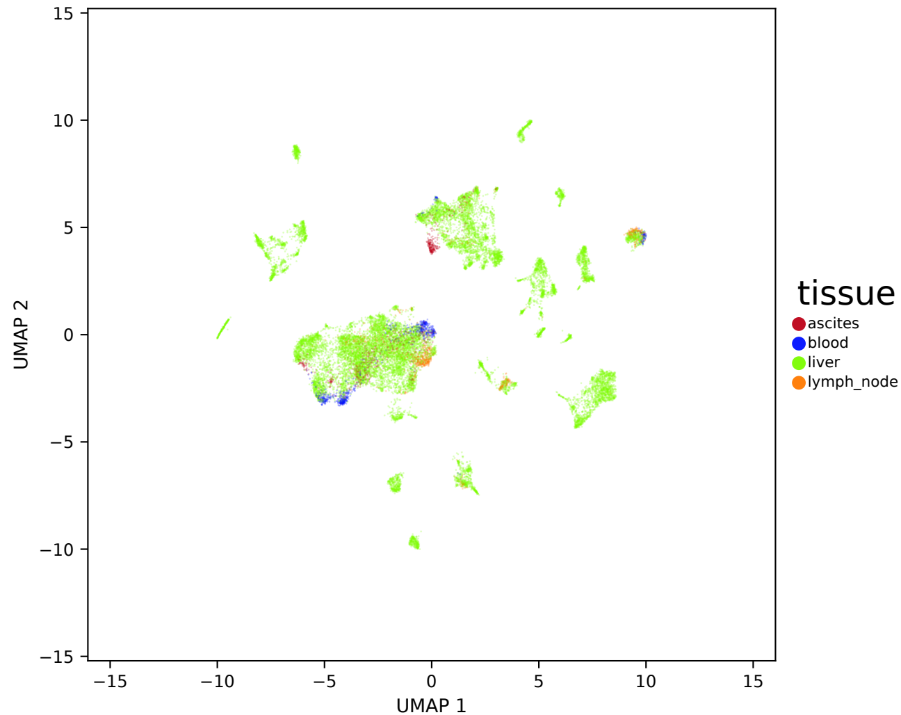
Scanorama — scanorama_smoke (n=19,997) — tissue
