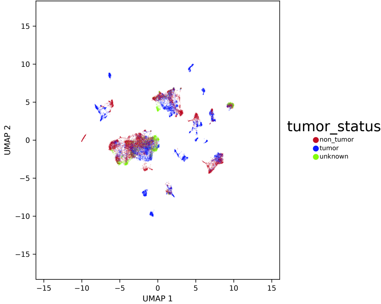
Scanorama — scanorama_smoke (n=19,997) — tumor status
