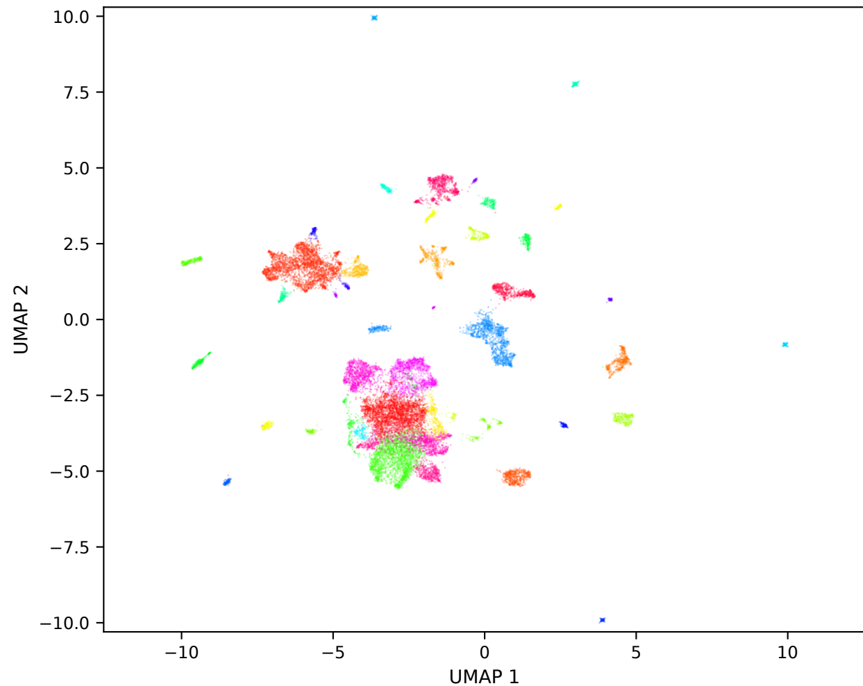
scVI — scvi_smoke (n=19,997) — leiden scvi smoke
