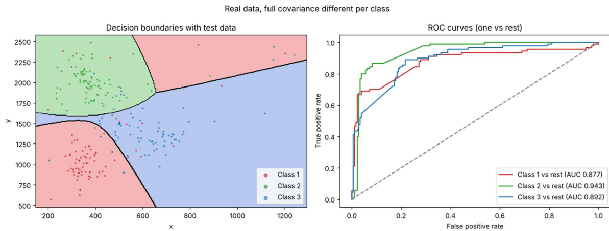
Figure 7. Real data: decision boundaries with the 270 test points (left) and ROC curves (right).
