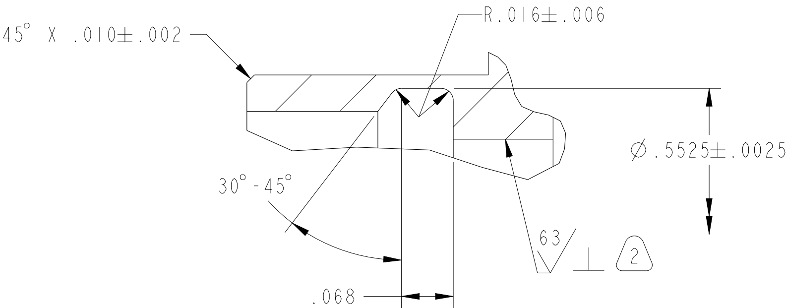
DETAIL E SCALE 8
