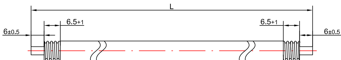
Drawing 1
