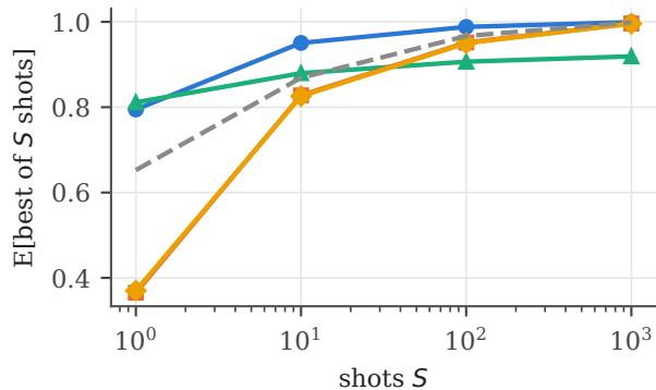
(b) best-of- S saturates, n = 12 , p = 3
