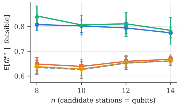
(a) single-shot quality, family R, p = 3
