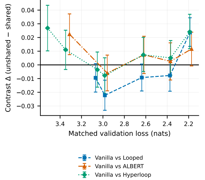
Figure 2: Difference between the unshared baseline and each weight-reusing encoder, at every matched point.
