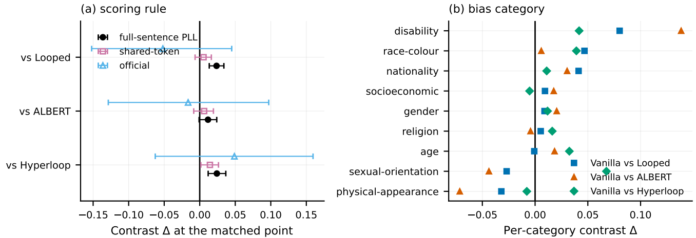
Figure 3: The same comparisons under (a) different scoring rules and (b) the nine bias categories.
