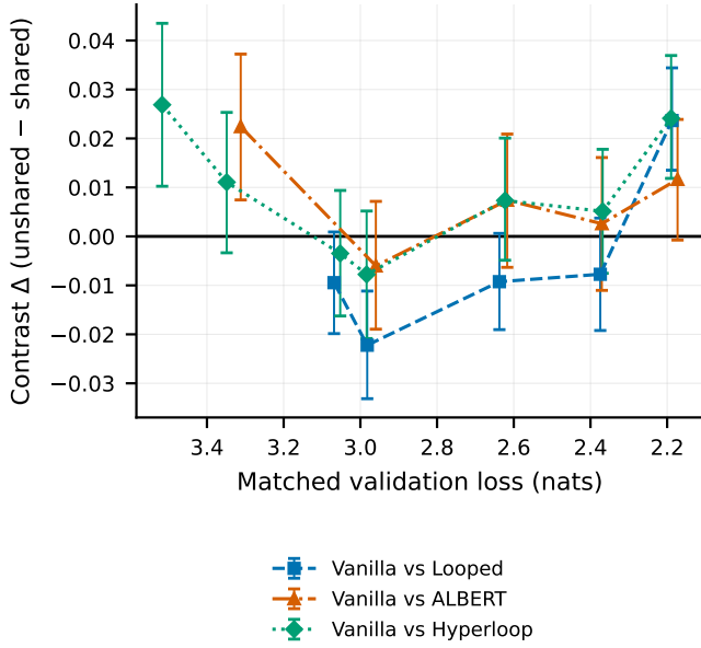
Figure 2: Difference between the unshared baseline and each weight-reusing encoder, at every matched point.
