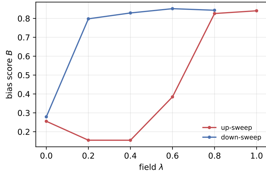
muril / hi / race-colour ( A = +0.363 , largest |A| )
