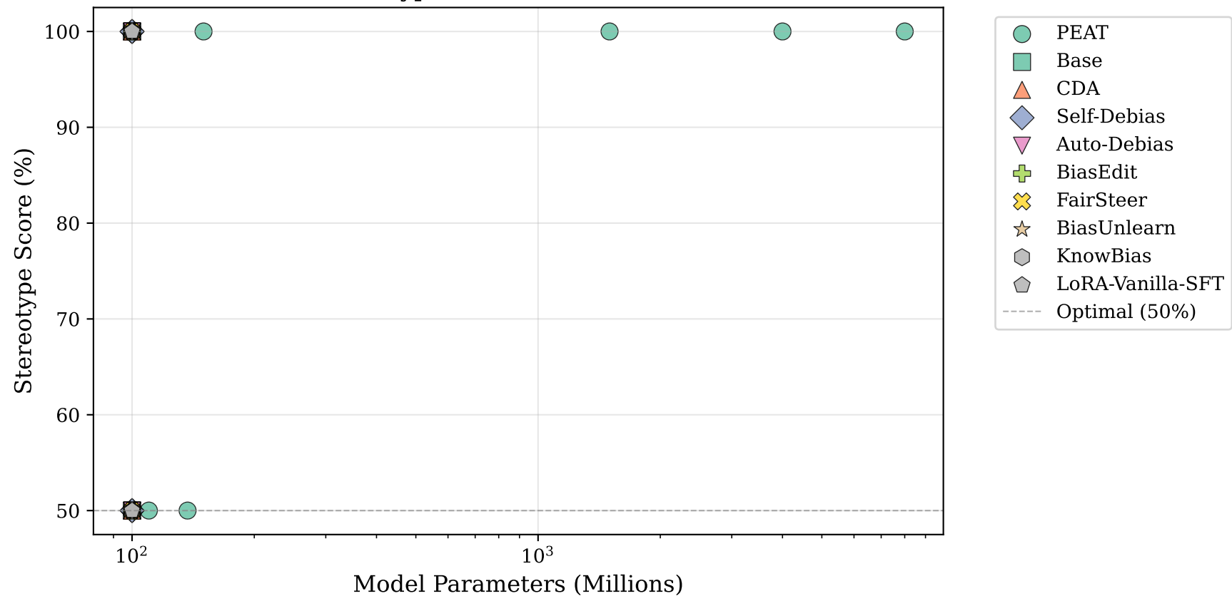
Stereotype Score vs. Model Scale
