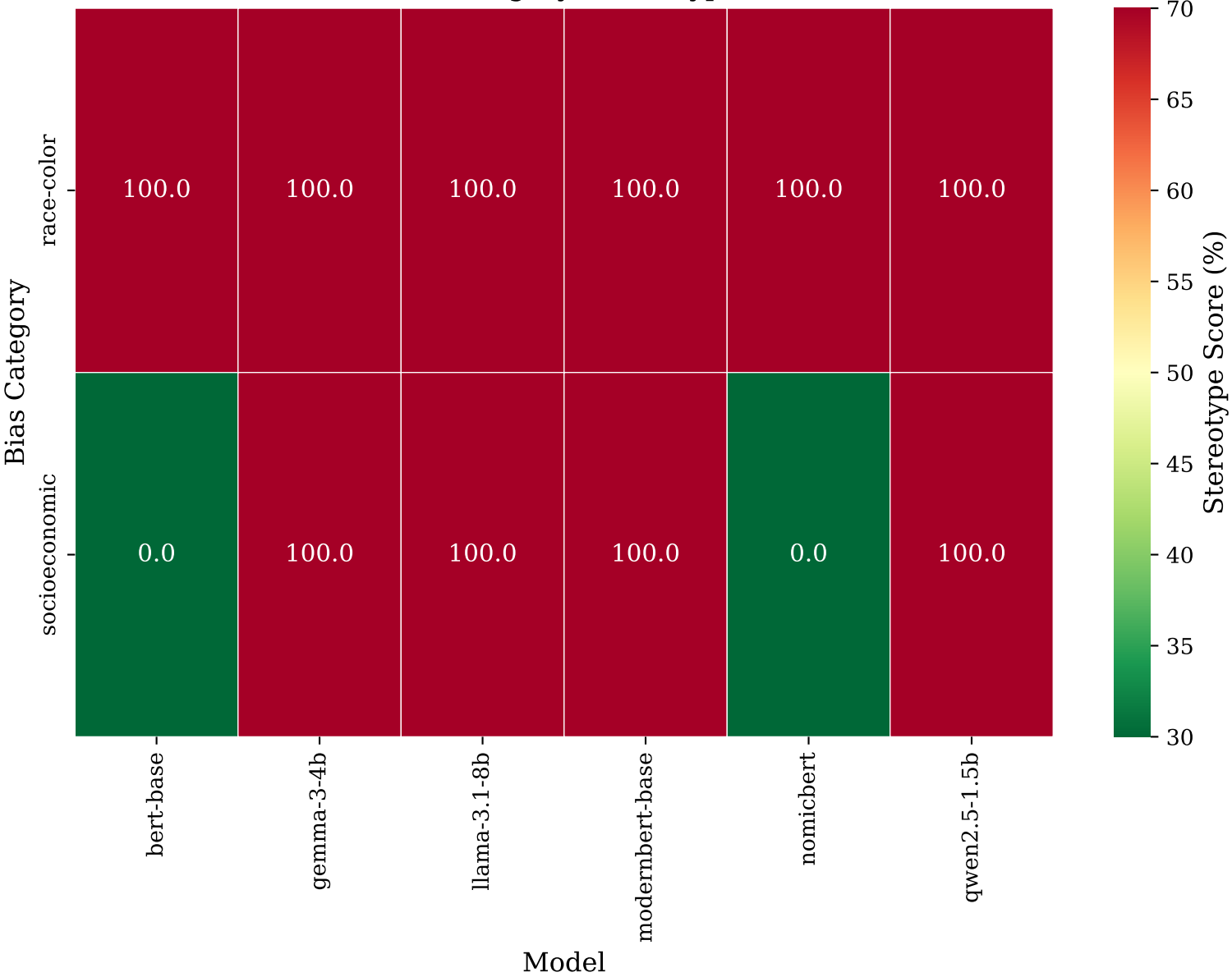
PEAT Per-Category Stereotype Score
