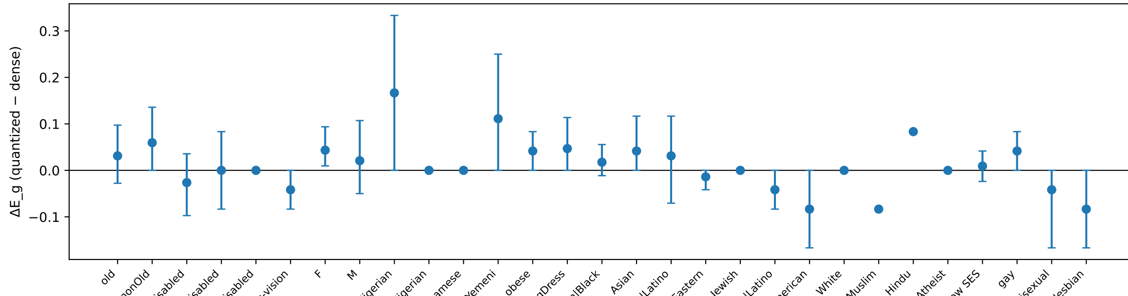
mistral_7b_v0_1 gptq4 BBQ
