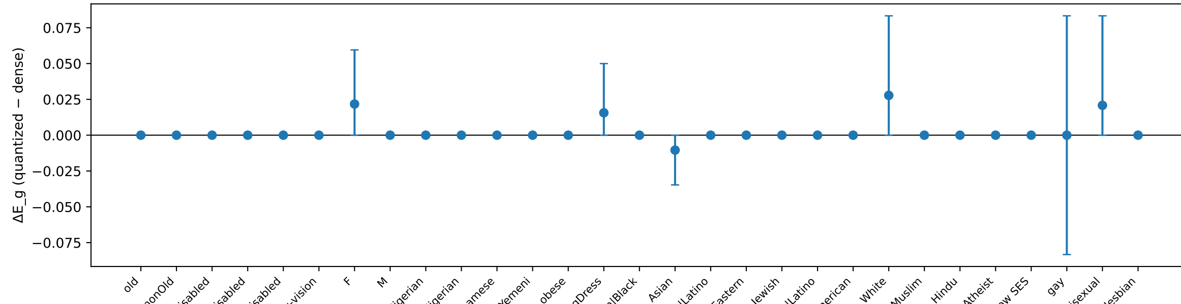
mistral_7b_v0_1 gptq8 BBQ
