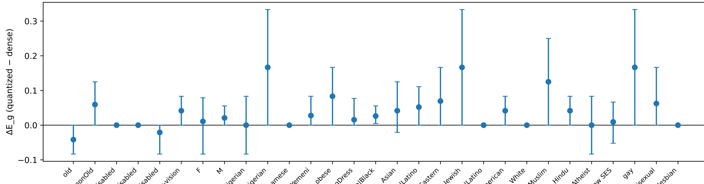
qwen3_8b rtn4 BBQ
