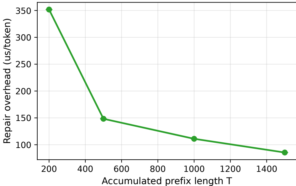
Repair Cost Scaling (LLaMA-2-7B)
