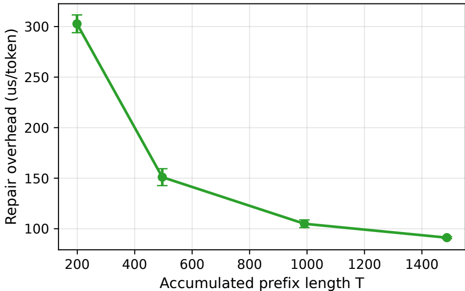
Repair Cost Scaling (Falcon-7B)
