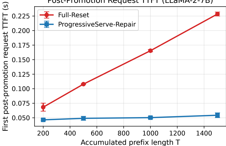
Post-Promotion Request TTFT (LLaMA-2-7B)
