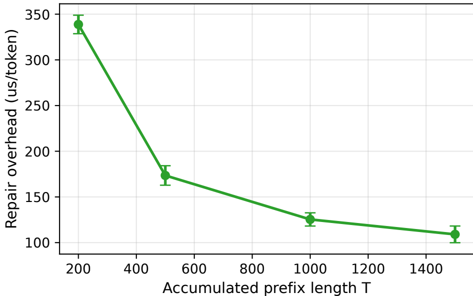
Repair Cost Scaling (LLaMA-2-13B)
