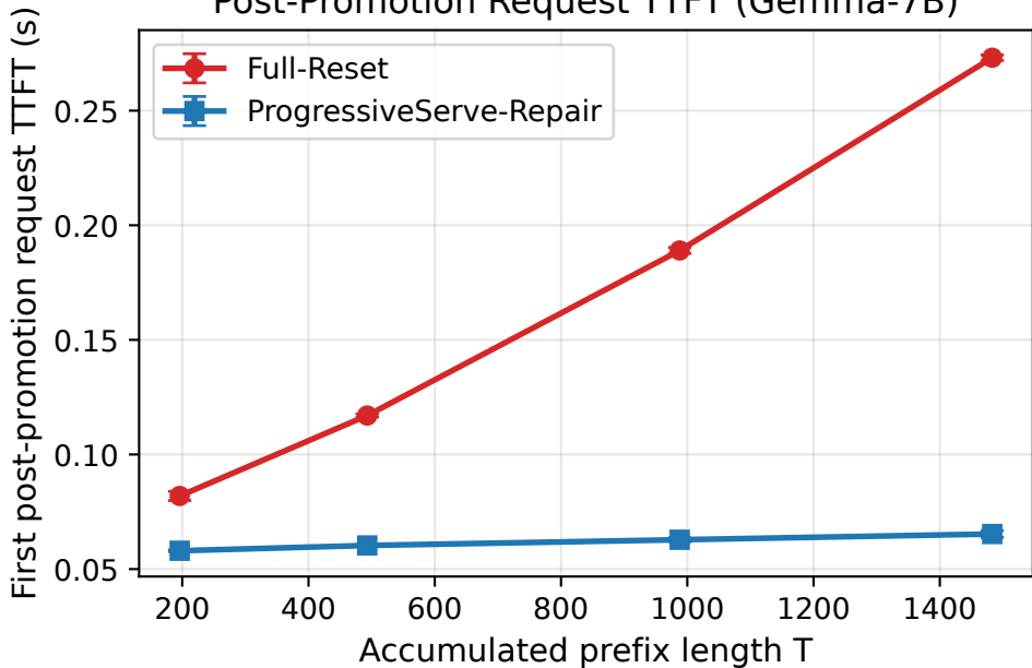
Post-Promotion Request TTFT (Gemma-7B)
