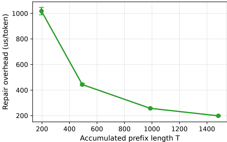
Repair Cost Scaling (Gemma-7B)
