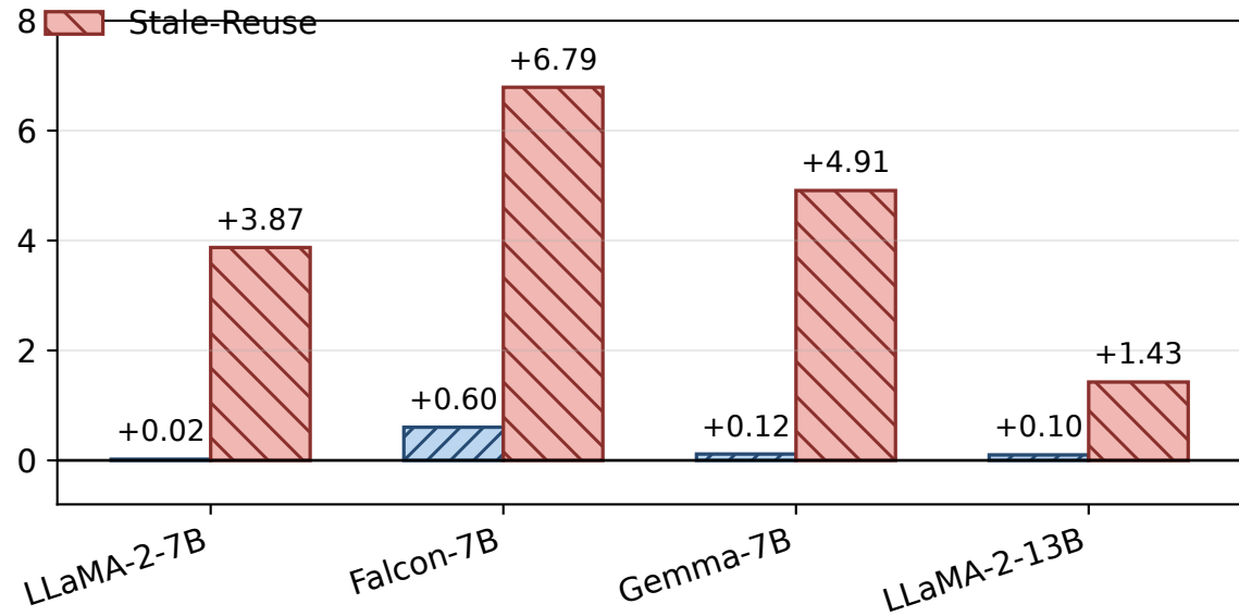
Delta PPL vs Oracle-Recompute
