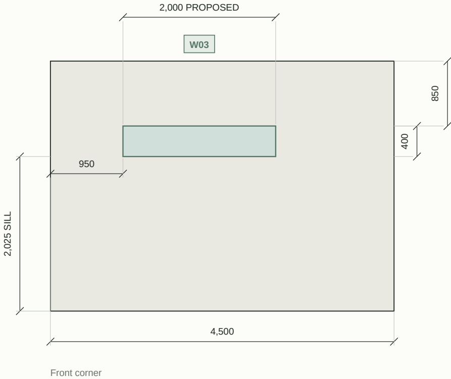
BEDROOM END ELEVATION
